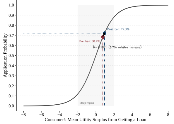
(a) Logistic CDF under No-Internalization
