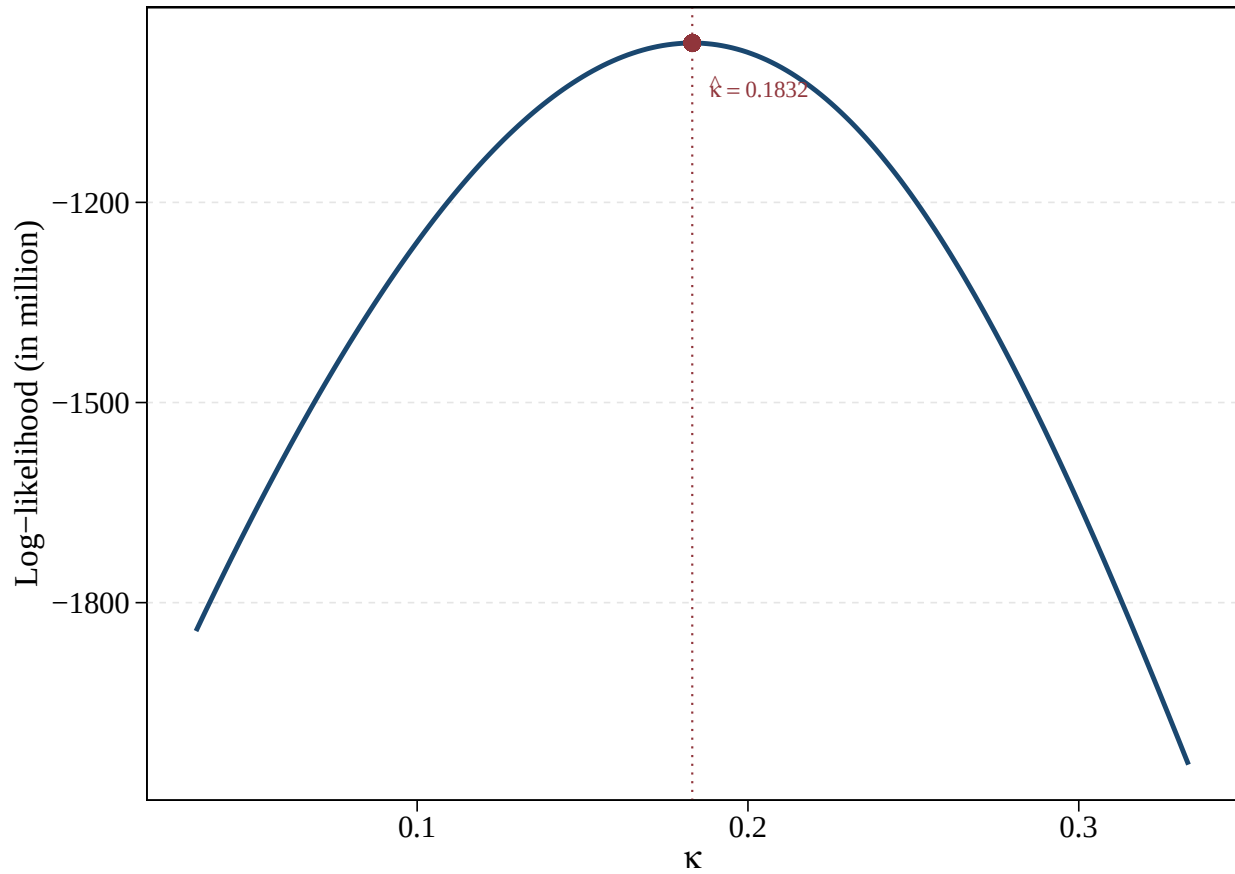
Figure E.1: Identification of \kappa : Log Likelihood Function
