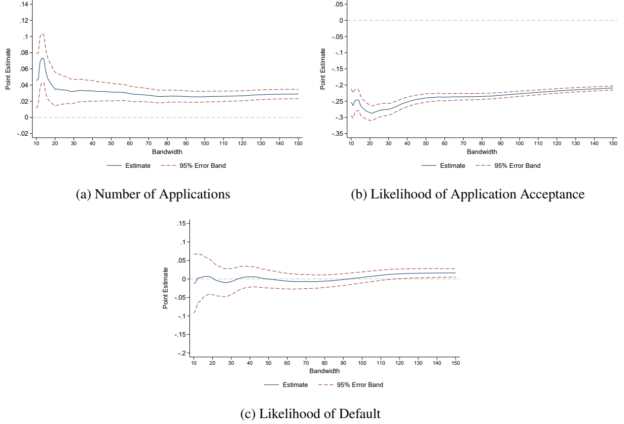
Figure C.1: Robustness to Bandwidth Choice: High-Frequency Event Study Estimates Across Multiple Bandwidths
