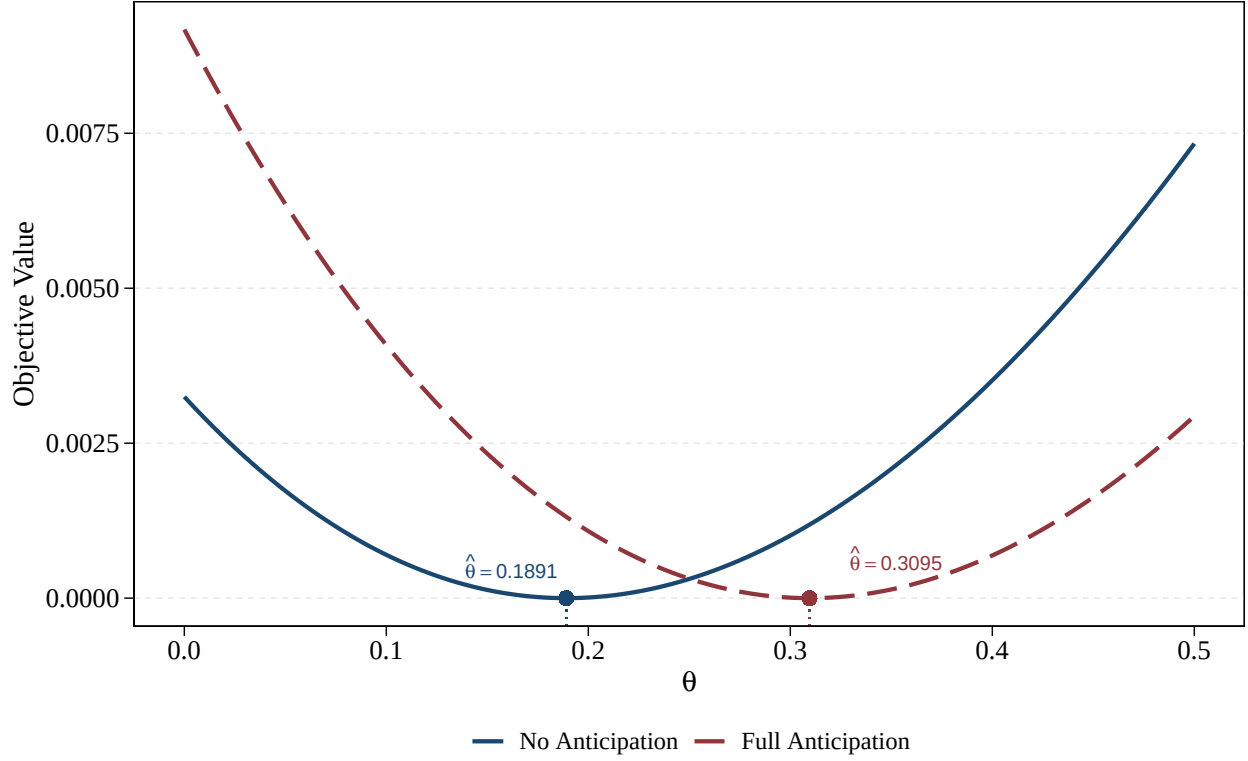
Figure E.2: Identification of \theta : Objective Function
