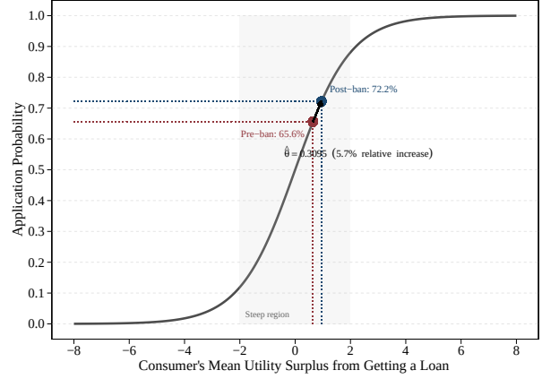
(b) Logistic CDF under Full-Internalization
